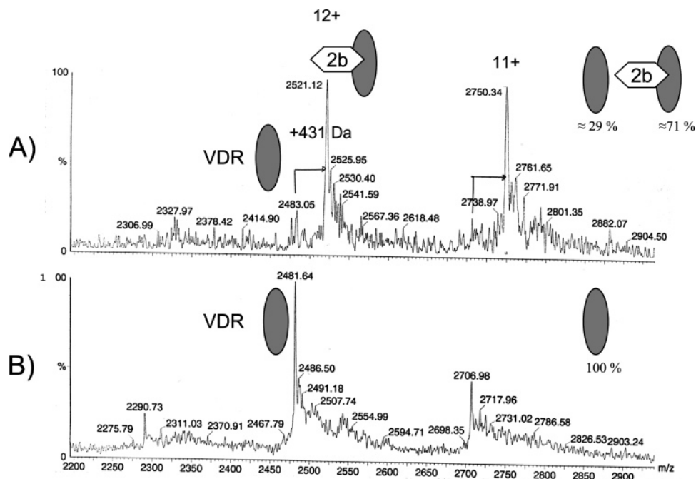
Figure 3. ESI mass spectra of hVDR LBD. The mass spectra were acquired at 20 V. (A) After addition of 3 molar equiv of 2b (MM = 431 Da). 71% of the detected species correspond to the hVDRΔ- 2b complex and 29% are related to unliganded VDR. (B) Before any ligand.
